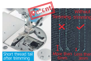
Initial sewing without bird nest; Short thread tail after trimming
